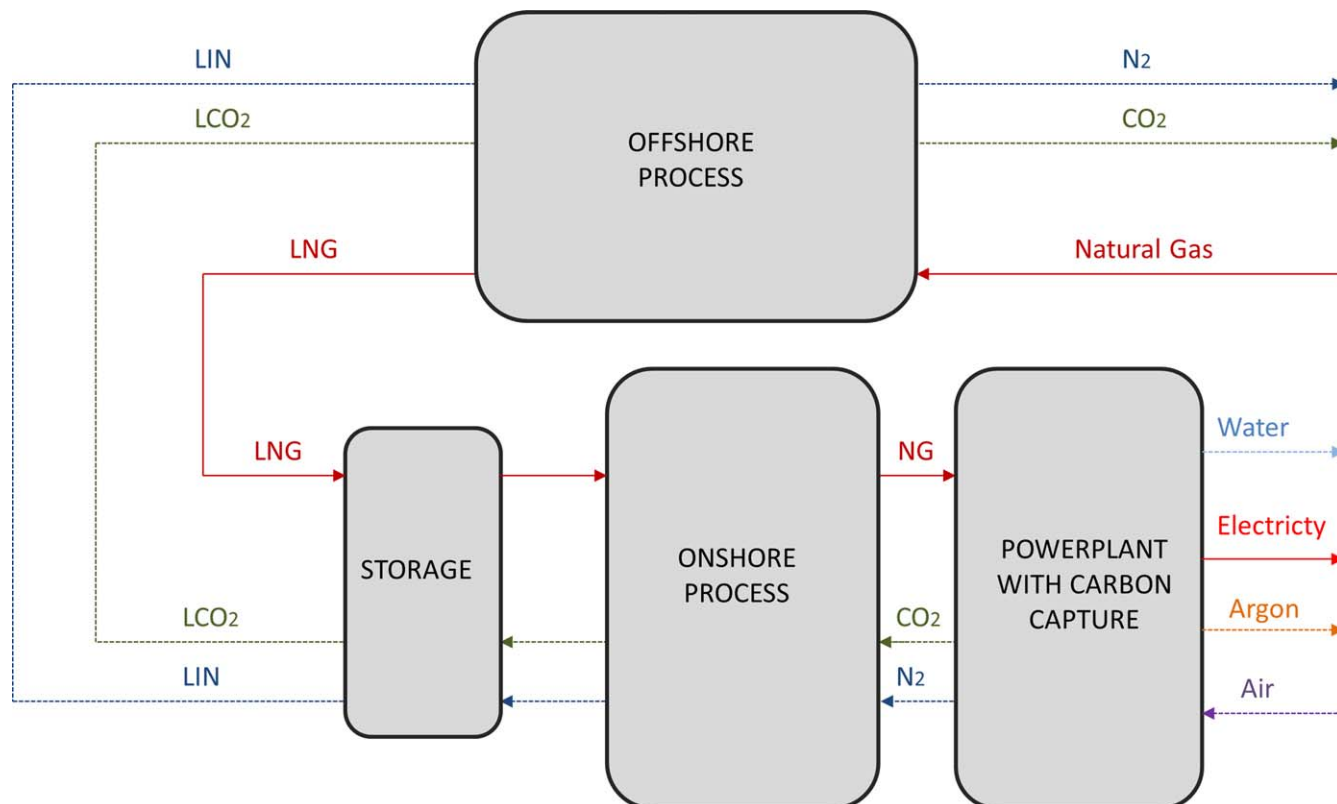
Figure 1. Energy chain for transport and utilization of LNG (From Wechsung et al., 3 reproduced by permission.).
