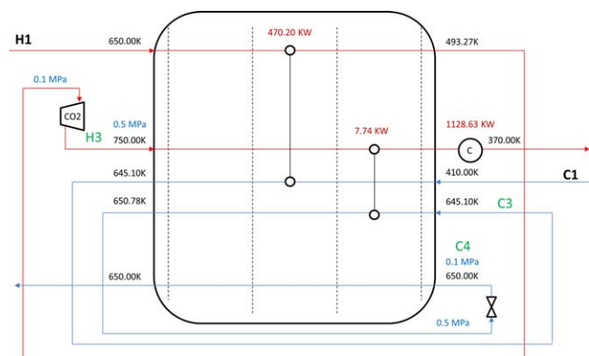
Figure 5. Optimal HEN configuration obtained for Example 1-Case 3.
