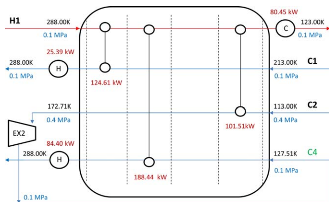
Figure 8. Optimal HEN configuration obtained for Example 2-Case 3.
