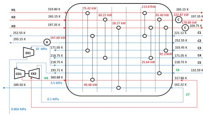
Figure 12. Optimal HEN configuration obtained for Example 3—Case 2.
