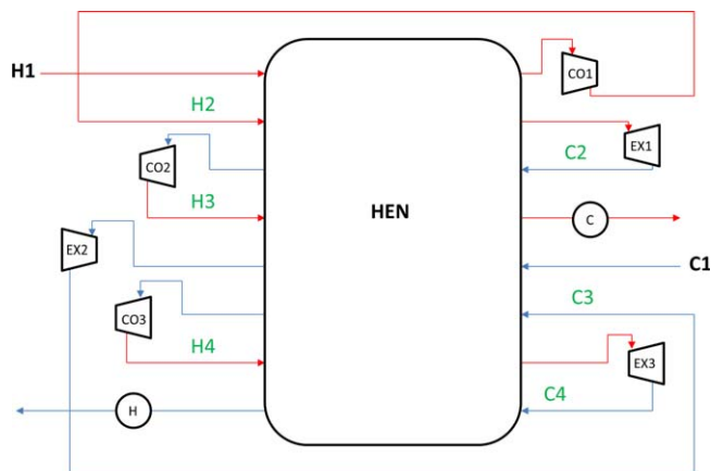
Figure 2. Possible streams arrangement for Example 1.
