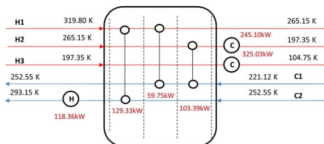
Figure 13. Optimal HEN configuration obtained for Example 3—Case 3.
