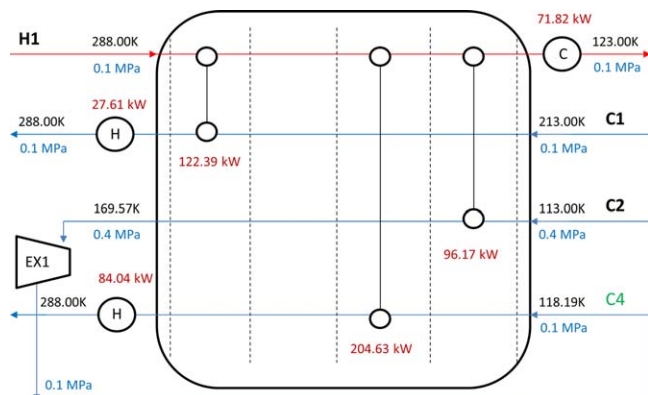
Figure 7. Optimal HEN configuration obtained for Example 2-Case 2.
