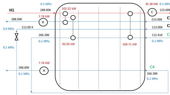
Figure 9. Optimal HEN configuration obtained for Example 2-Case 4.
