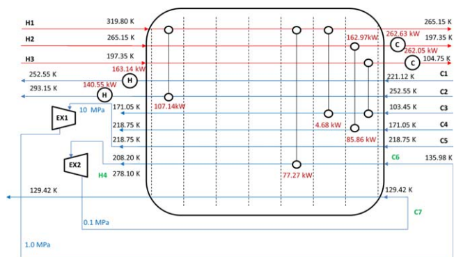
Figure 11. Optimal HEN configuration obtained for Example 3-Case 1.
