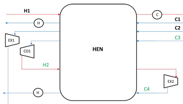
Figure 6. Possible streams arrangement for Example 2.
