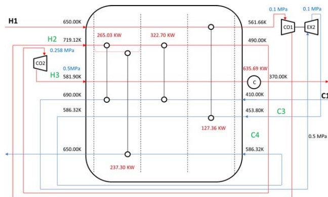
Figure 4. Optimal HEN configuration obtained for Example 1-Case 2.
