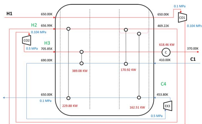
Figure 3. Optimal HEN configuration obtained for Example 1–Case 1.
